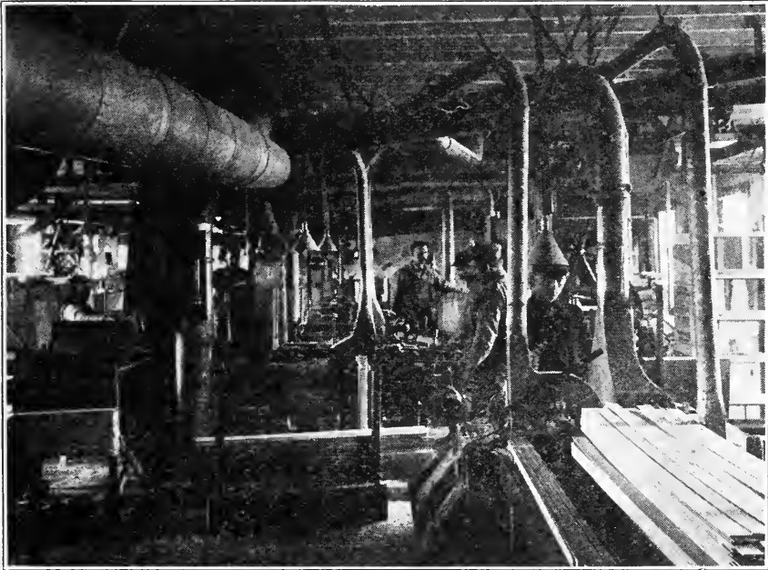
FIG. 232 . EXHAUST SYSTEM—INTERIOR PIPING.
